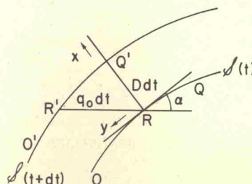
FIG. 1. Shock front produced by steady disturbance at O.
